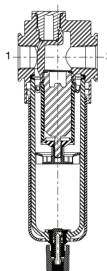
Cross Section - 651/652/653 Series Particulate Filter
