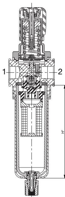
Cross Section - 651/652/653 Series Coalescing Filter/Regulator
