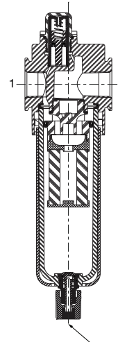
Cross Section - 651/652/653 Series Coalescing Filter
