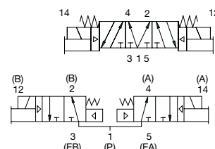
double solenoid air pilot 3 position 4-way pressure center
