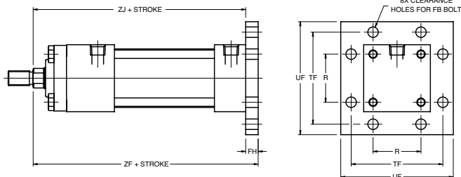
1-1/2" Thru 2-1/2" Bore
