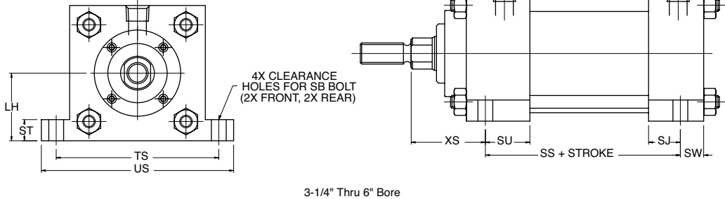
Mount Code S2
