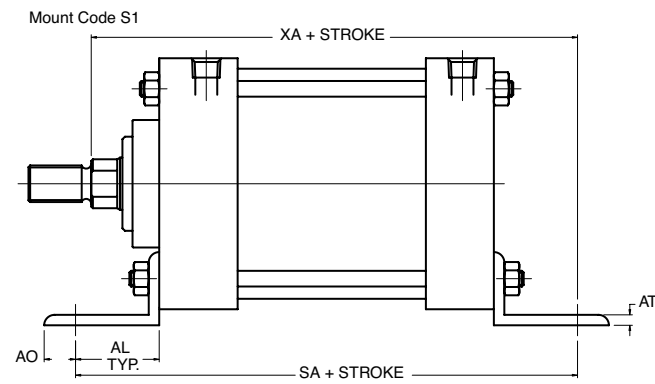
3-1/4" Thru 6" Bore
