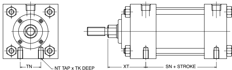
3-1/4" THRU 8" BORE
