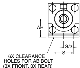
1-1/2" Thru 2-1/2" Bore
