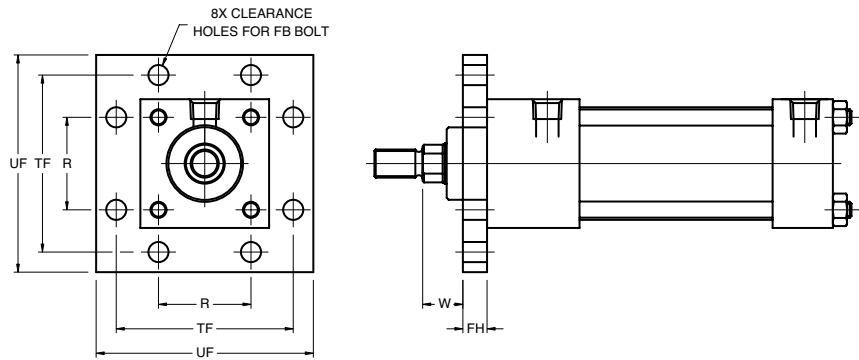
Mount Code F5
