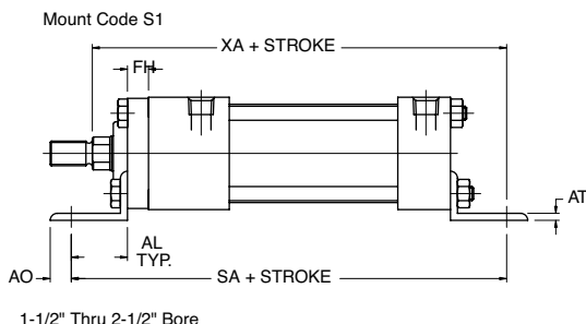
1-1/2" Thru 2-1/2" Bore
