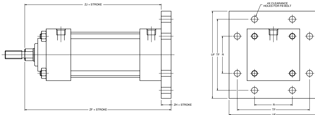
3-1/4" Thru 6" Bore
