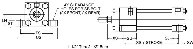
Mount Code S2
