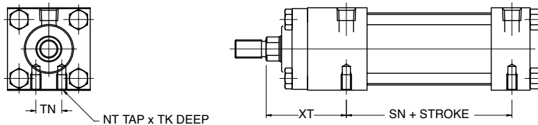
1-1/2" Thru 2-1/2" Bore
