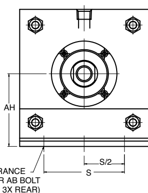
3-1/4" Thru 6" Bore
