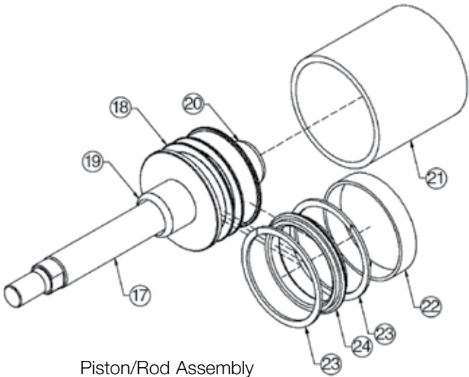
Piston/Rod Assembly
