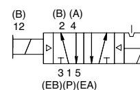
SPA double solenoid air pilot 2 position 4-way
