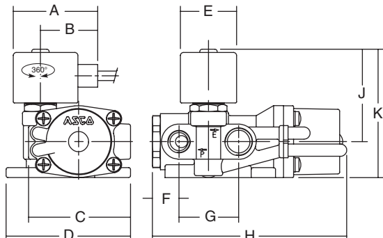
TYPE 09 Epoxy encapsulated EF: ICS-6 ANSI / NEMA Type 7 and 9 NOTE: applicable to solenoid only
