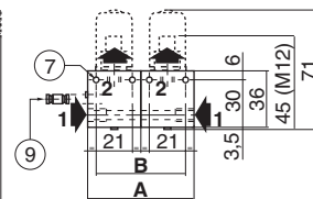
TYPE 05 Joinable subbase Zamak 35300048
