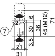
TYPE 04 Single subbase Zamak 35300047
