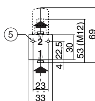
TYPE 04 Single subbase Zamak 35300047
