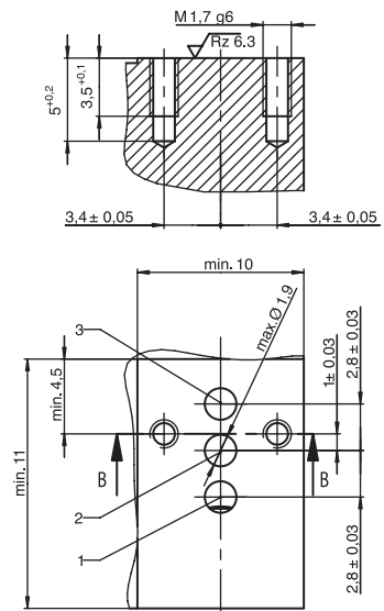
flange facing
