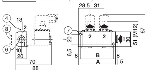
TYPE 03 Joinable instant fitting subbase Polyamide 35300070 35300071 (set of 2)
