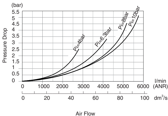
St. steel Filter 1/4 NPT Ref. : 342A9001 Filtration 25 µm with P inlet 4 - 6,3 - 8 - 10 bar
