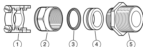
1 cable clamp 2 nut 3 backup ring 4 grommet 5 adapter (1/2 or 3/4 NPT)
