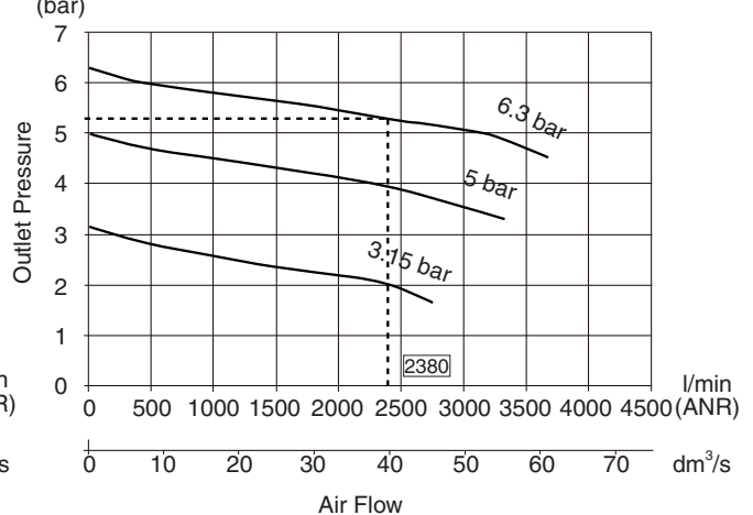
St. steel Filter Regulator 1/4 NPT Ref. : 342A8205 Filtration 5 µm with P inlet 10 b - setpoint 3,15 - 5 - 6,3 bar
