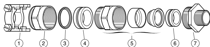
1 cable clamp 2 nut 3 backup ring 4 grommet (internal sealing) 5 armour clamp 6 grommet (external sealing) 7 adapter (1/2 or 3/4 NPT)
