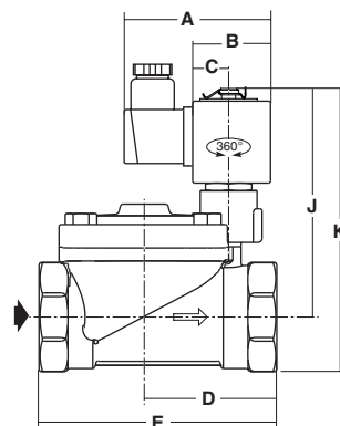
TYPE 03 Prefix "SC" Solenoid Black PPS moulded IEC 335 / ISO 4400 IP65
